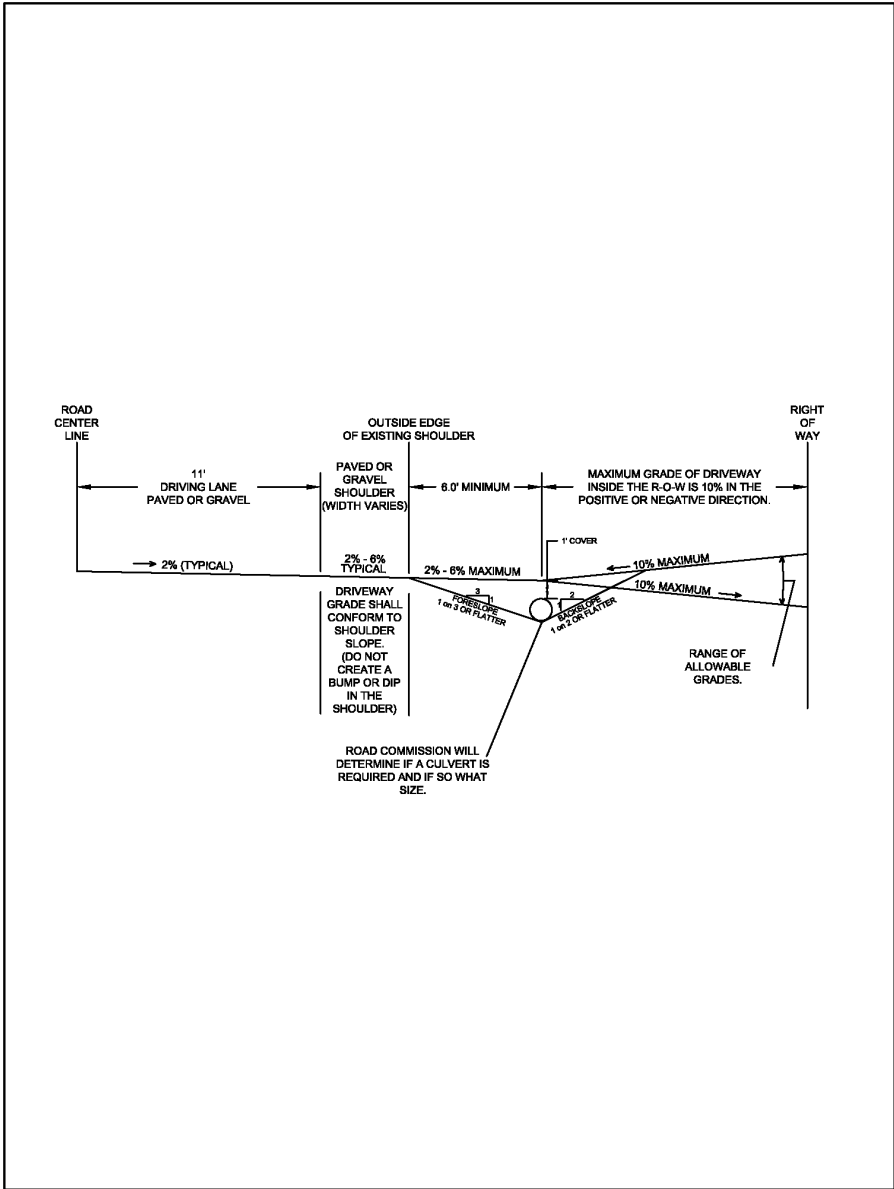
Figure 3: Driveway Profile Other Than Commercial
