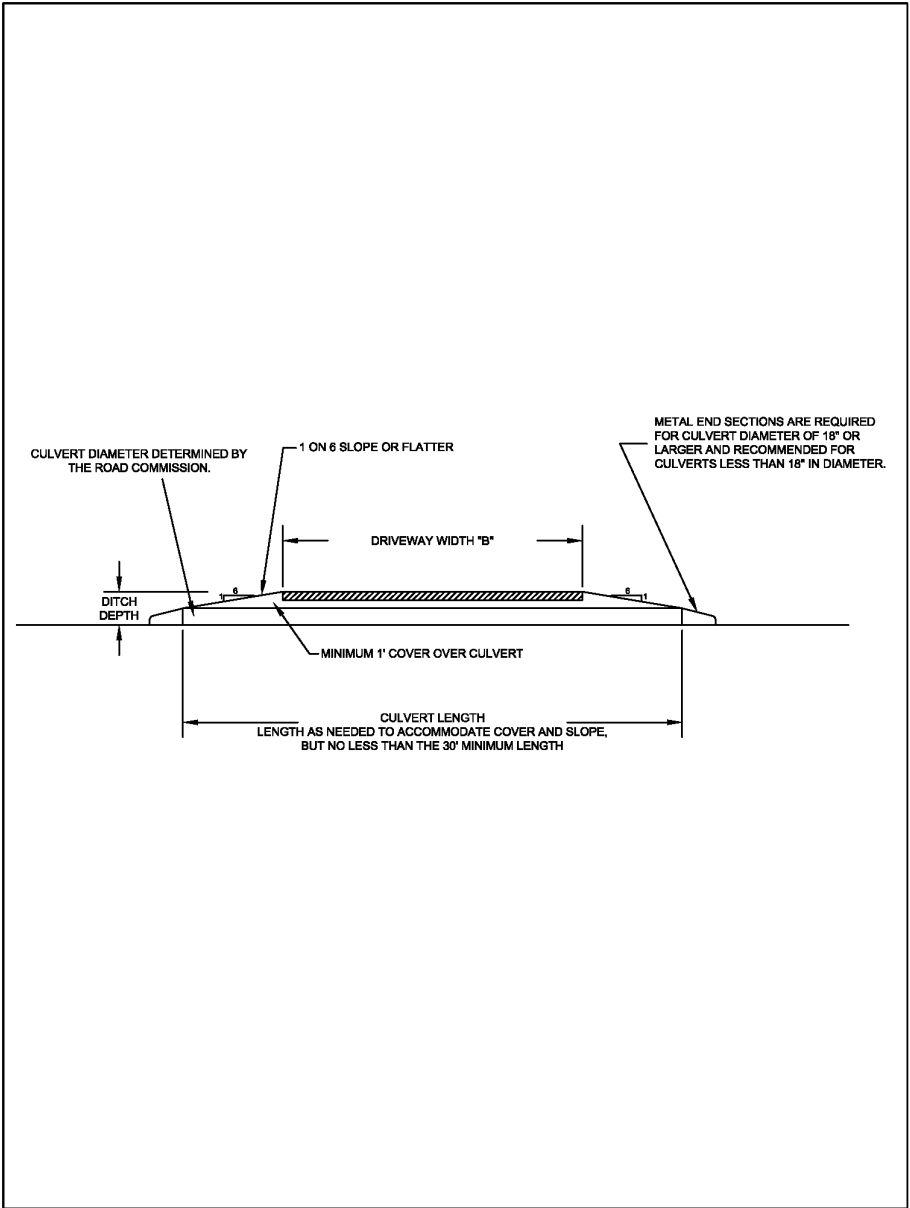
Figure 5: Driveway Cross Section
