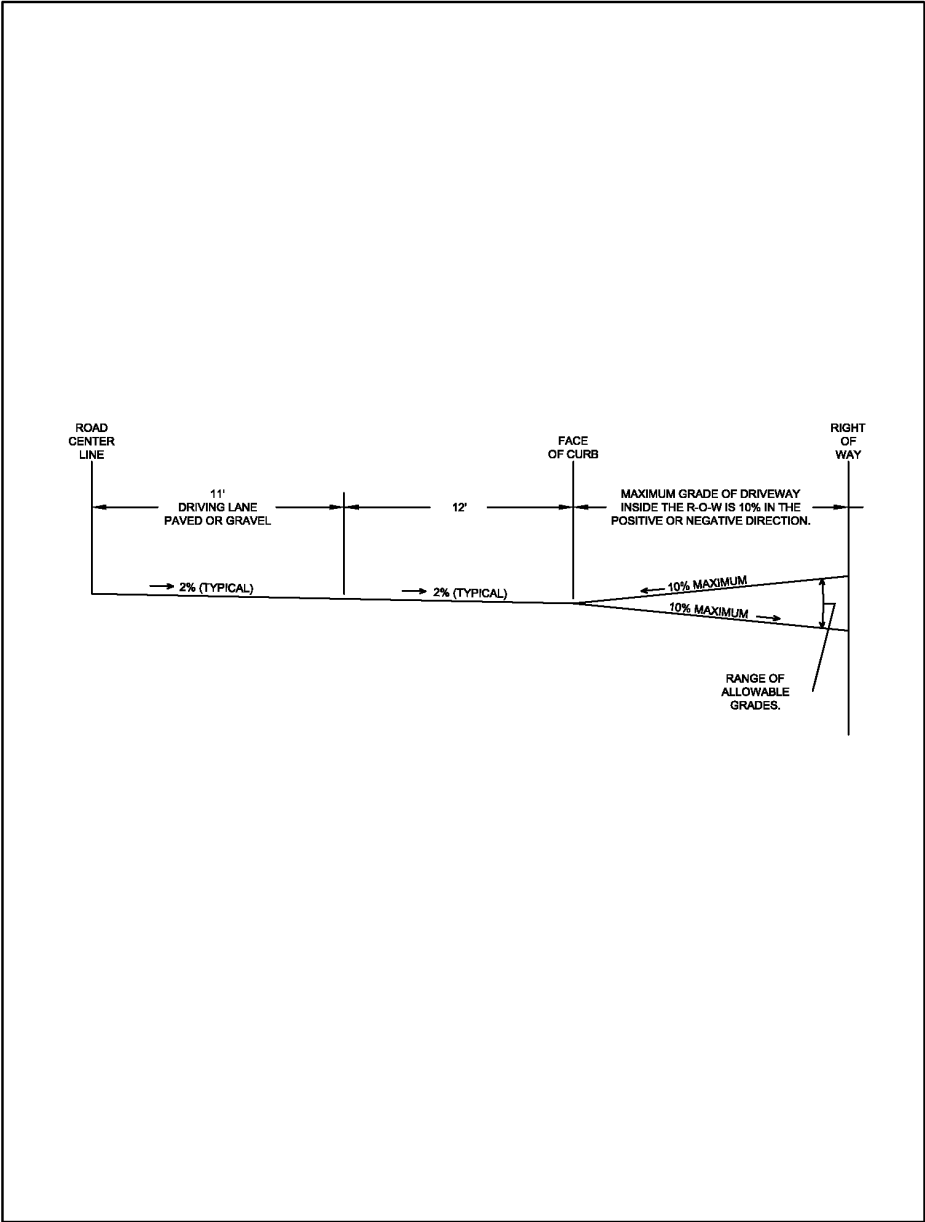
Figure 4: Driveway Profile Commercial
